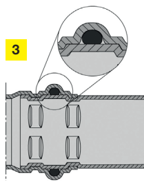
3 The double-pressed Viega fitting guarantees long-lasting security.
